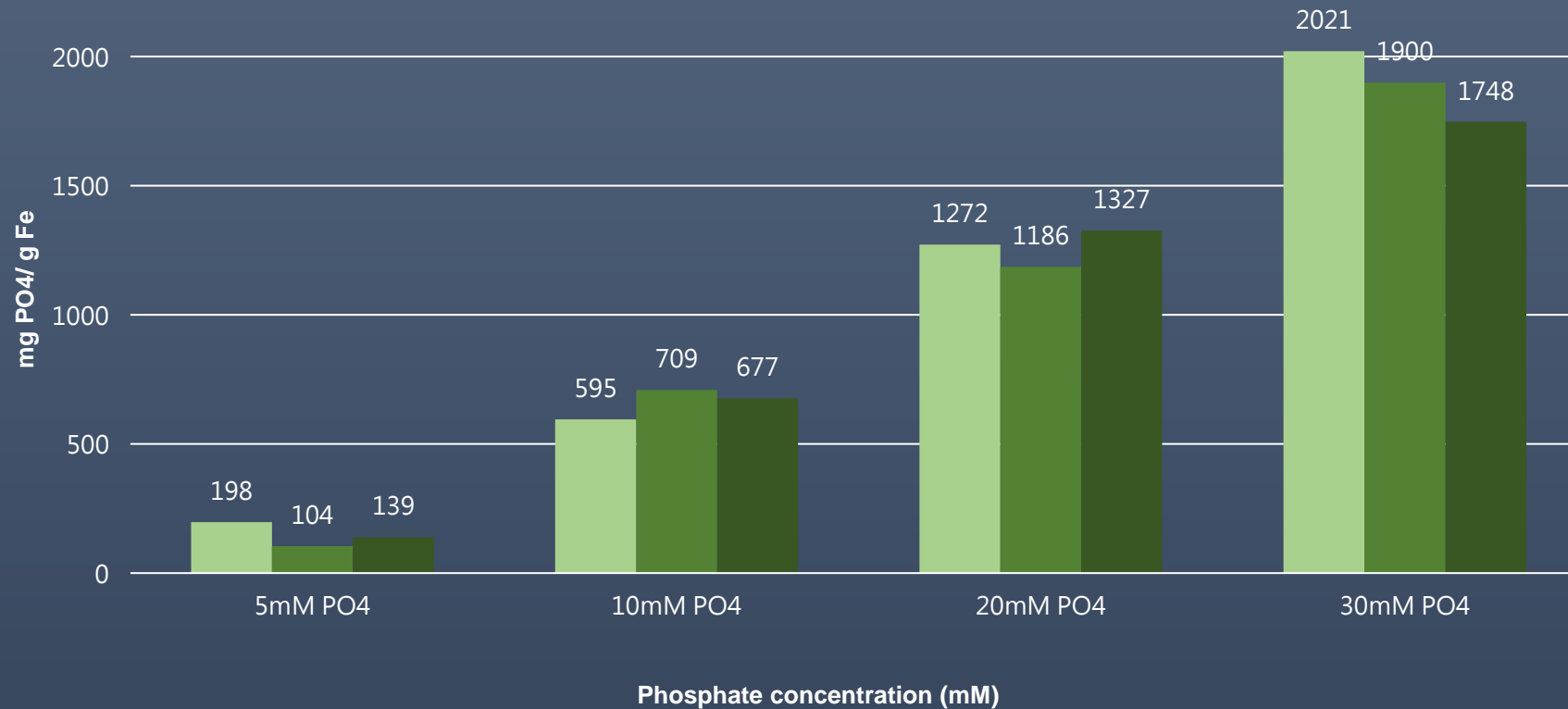
Oral Ferric citrate solution PO 4 binding capacity
